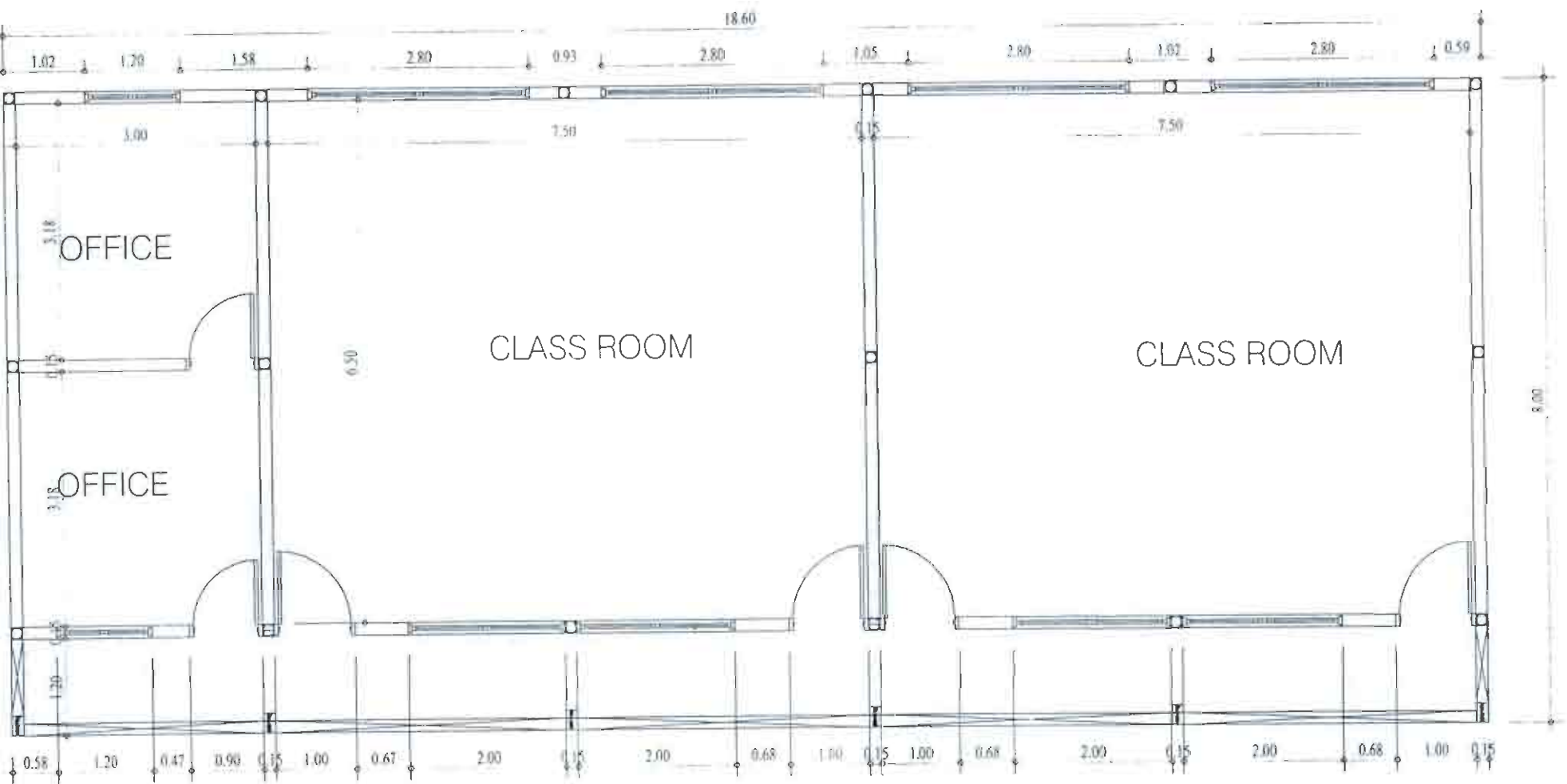
DISTRIBUTION PLAN
