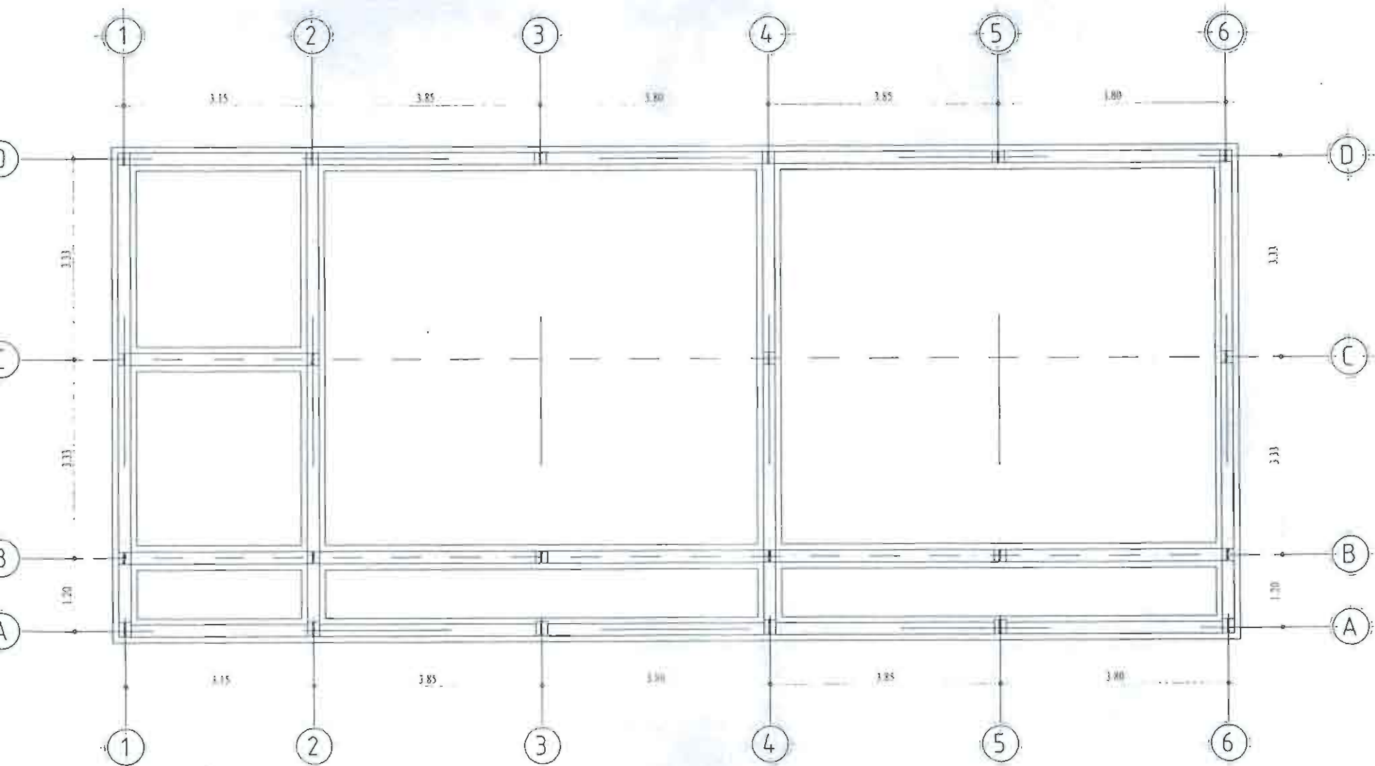
FOUNDATION PLAN
